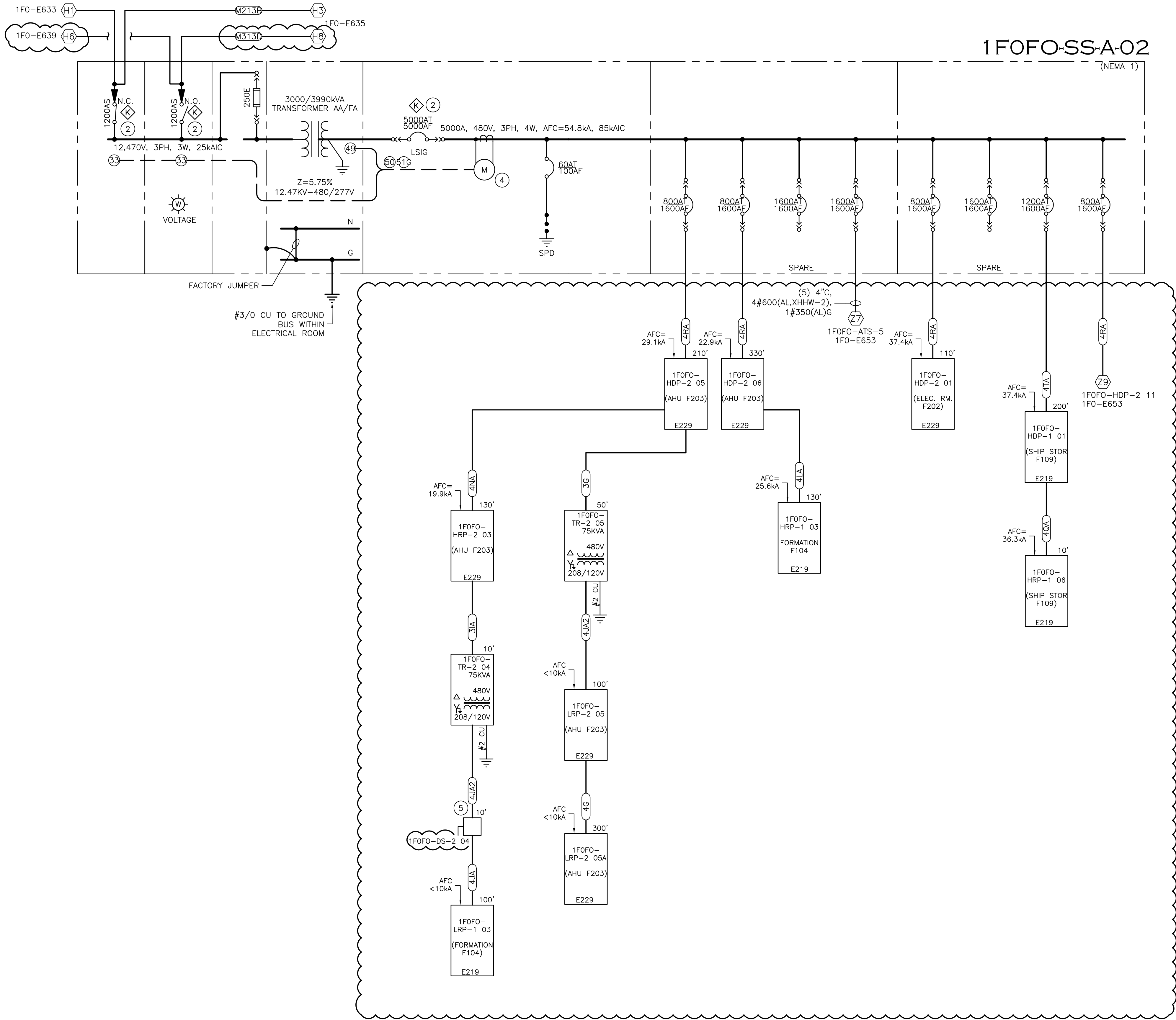
1 ONE LINE DIAGRAM - (1FO) FORMATION-1 "A" (PARTIAL) NO SCALE
